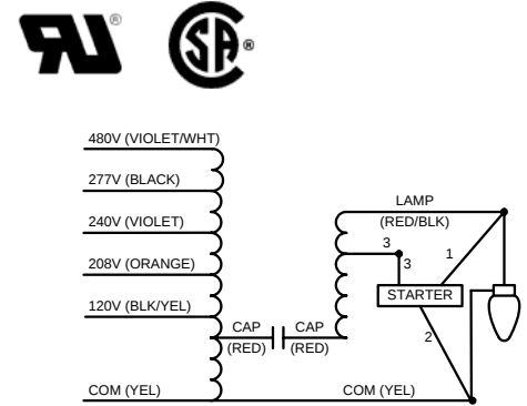
Optional 120V Standby Lamp 250 Watts Max.
